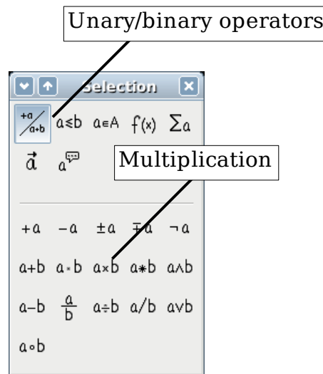
Figure 3. Unary/binary operators
